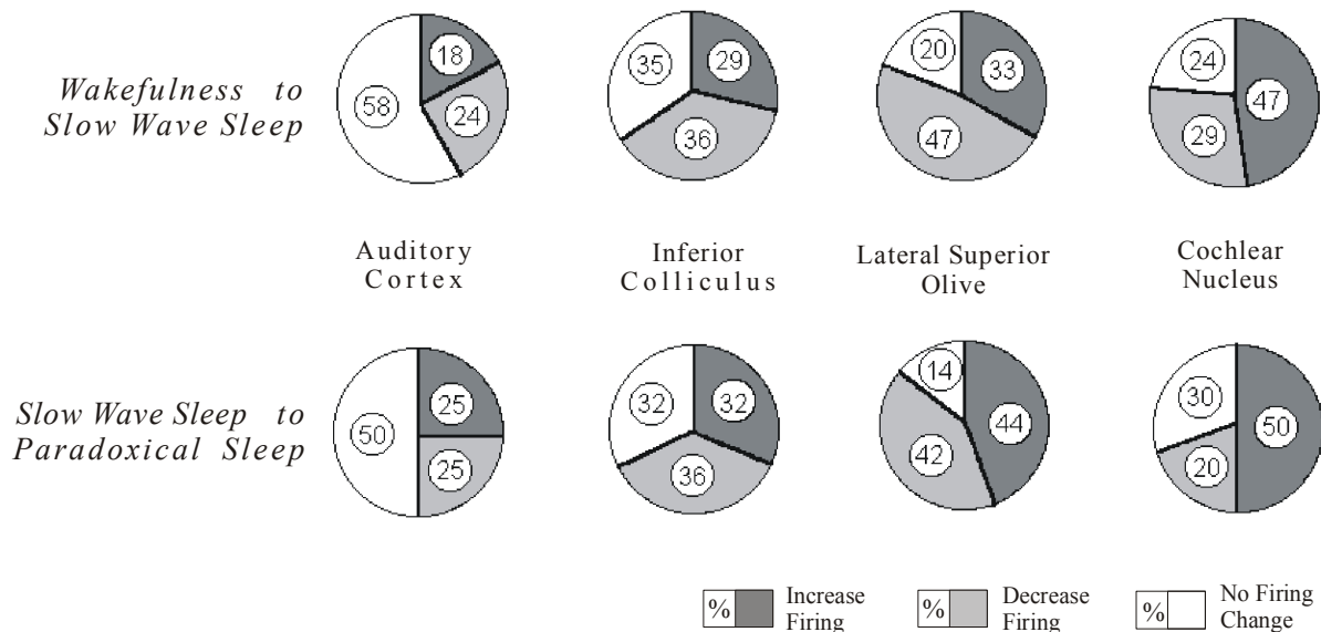
Figure 2. Guinea pig unitary evoked activity ( n=293 ) along the auditory pathway in the sleep-waking cycle. Pie charts show percentages of neuronal firing shifts on passing from Wakefulness to Slow Wave Sleep and from Slow Wave sleep to Paradoxical Sleep. The lower the locus the majority the increasing-decreasing firing neurones. No silent neurone was detected on passing to sleep or during sleep in any pathway level. Data from see 16 .
